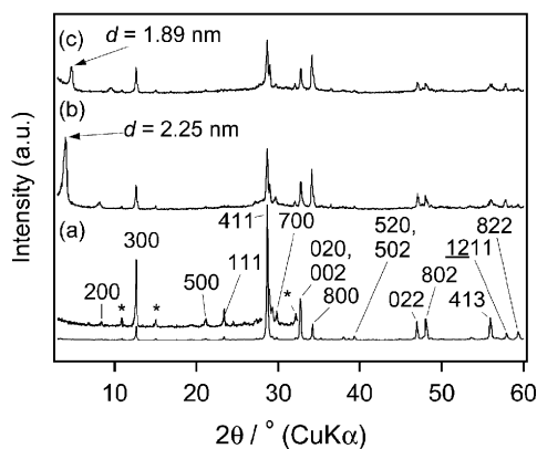
Fig. 1. The XRD patterns of (a) \text{Bi}_5\text{Nb}_3\text{O}_{15} , (b) the acid-treated product after drying at room temperature and (c) the acid-treated product after drying at 120 °C. Unindexed reflections are marked with asterisks.
